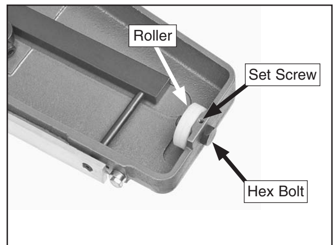
Figure 24. Rip fence height adjustment.
